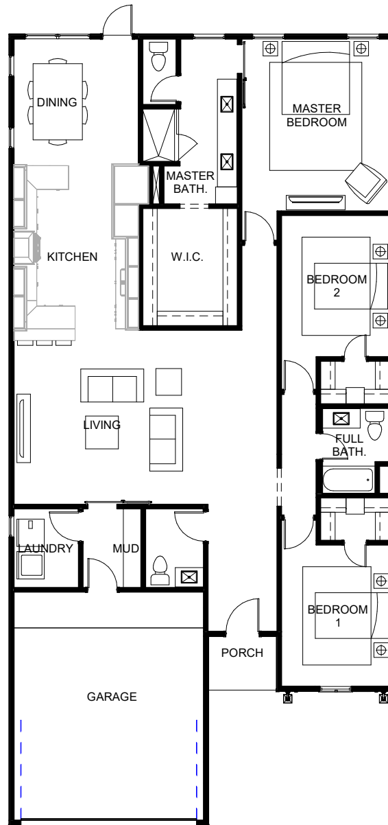
Floorplan
